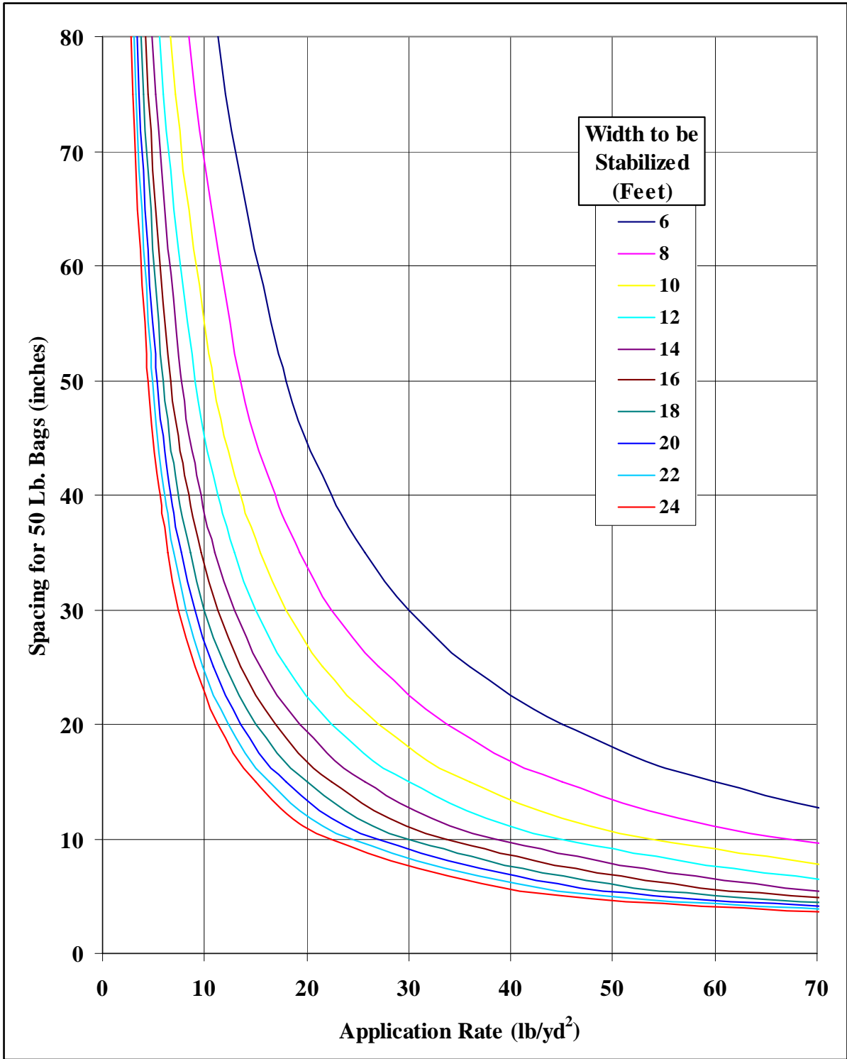
Figure 26: Bag Spacing
